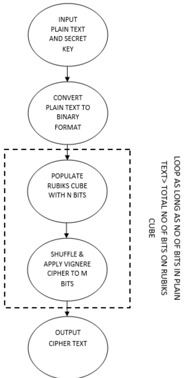
Fig 2. Proposed Method for Binary Encryption using Rubik's Cube Technique.
